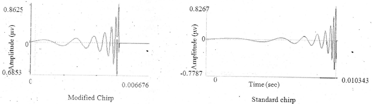
Figure 1: Temporal representation of modified chirp and standard chirp.
